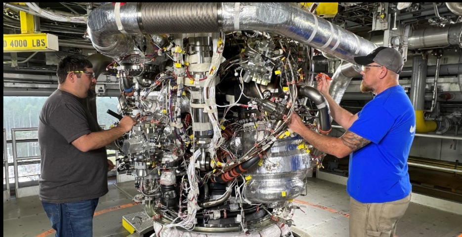
Artemis V & Beyond RS-25 Certification Testing Underway
